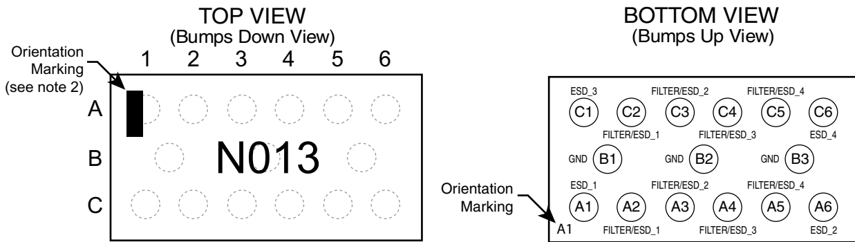
CM1401-03 CSP Package
